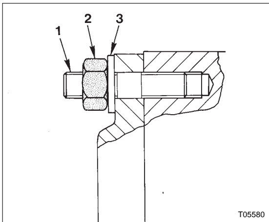
Figure 1 : Former half shaft flange installation (model 11.36)
