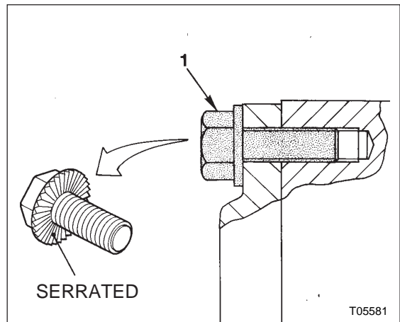
Figure 2 : Current half shaft flange installation (model 11.36)
