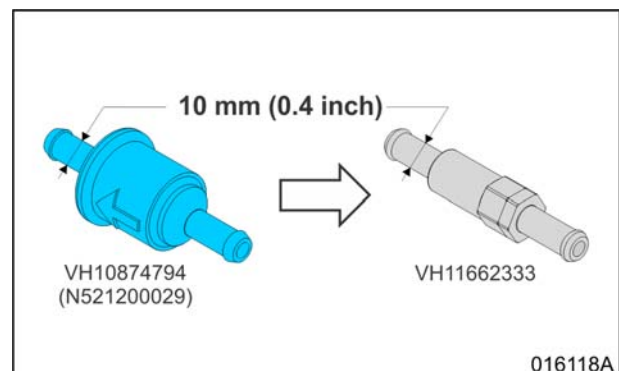
Figure 2: Single check valve 10874794 is replaced by 11662333
