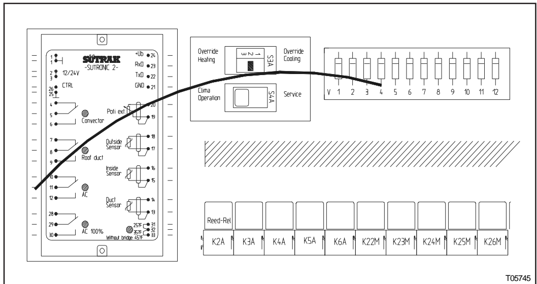
Figure 2: Jumper wire installation on the HVAC switchboard for PDI purposes (C2045 - Sytronic 2)
