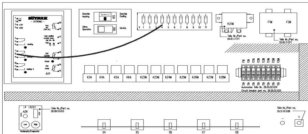
Figure 1: Jumper wire installation on the HVAC switchboard for PDI purposes (T2145 - Sytronic)
