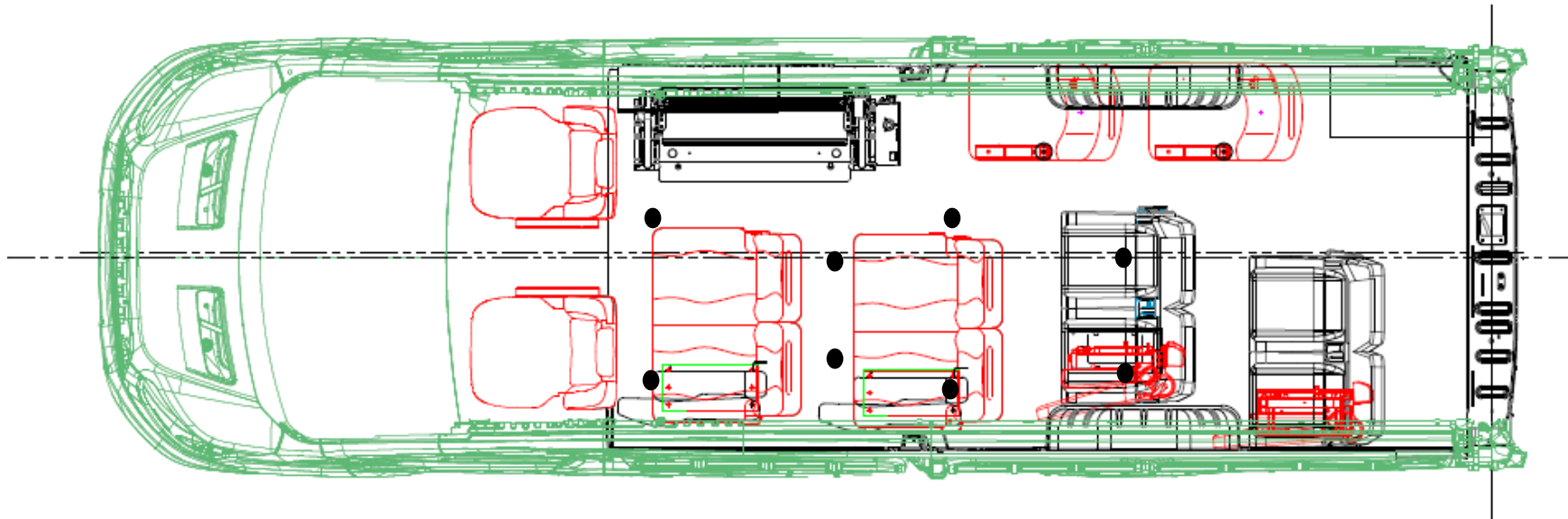
Curb Smart Van (Wood Floor) with Side Lift, Rear Single Bus Door Entry. 10 Ambulatory Rear Passengers and 2 Wheelchair Positions.
